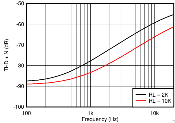
V_S = 5.5 \text{ V}, V_{CM} = 2.5 \text{ V}, G = 1, BW = 80 \text{ kHz}, V_{OUT} = 0.5 V_{RMS}
