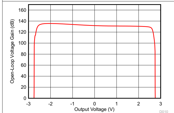
Figure 6-5. Open-Loop Gain vs Output Voltage
