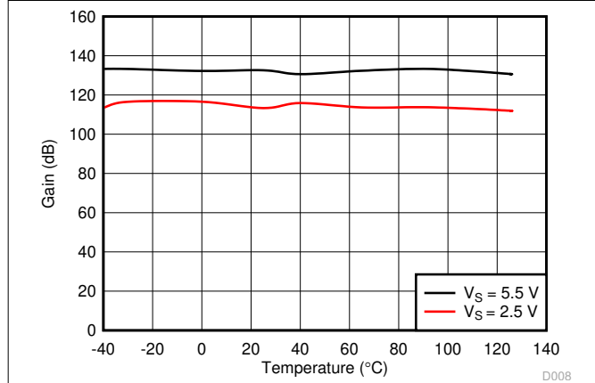
Figure 6-3. Open-Loop Gain vs Temperature
