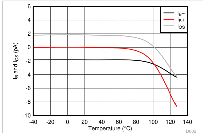
Figure 6-1. I_B and I_{OS} vs Temperature
